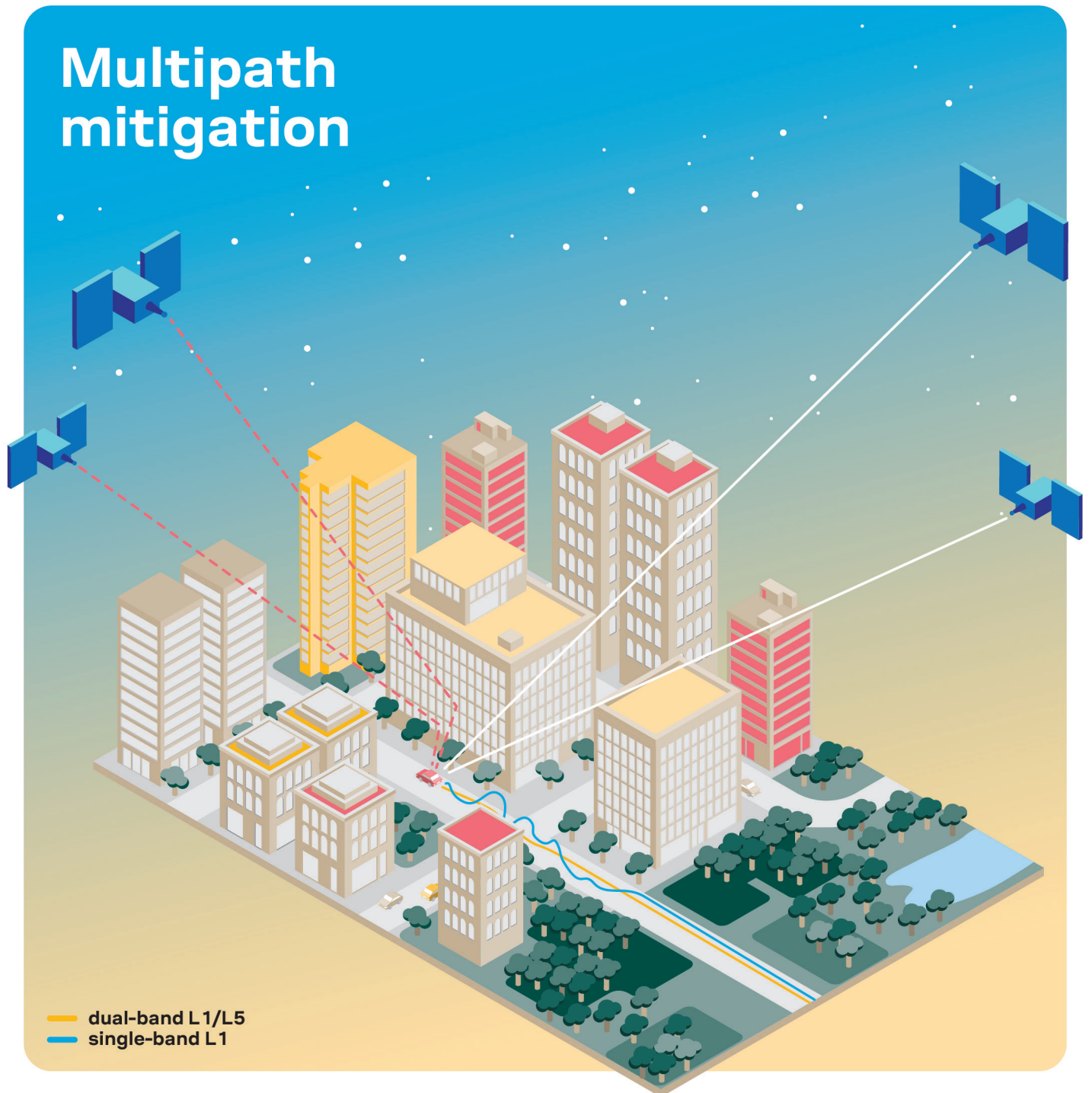
Figure 3. Larger GNSS position errors in an urban multipath environment
