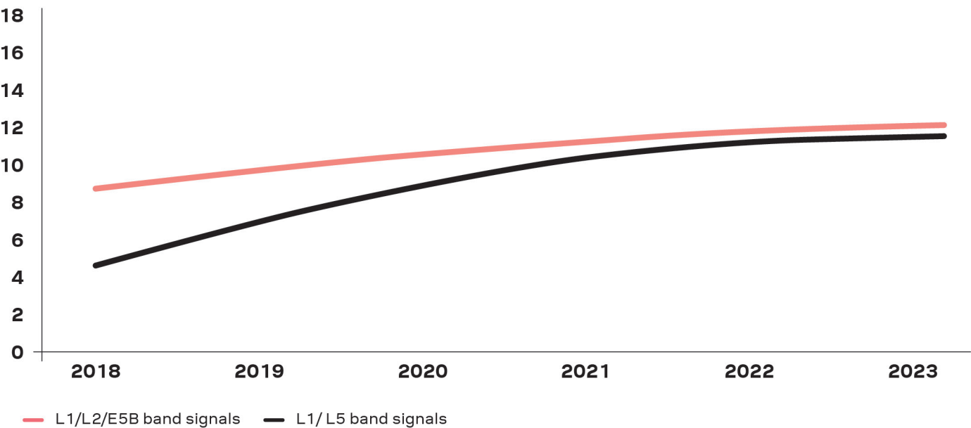
Figure 8. GNSS visibility over time
