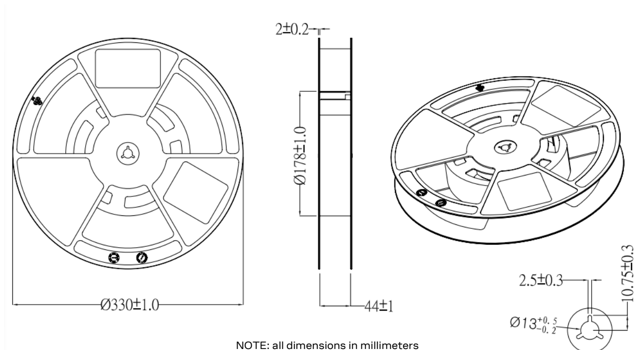
Figure 6: LENA-R8 series modules reel
