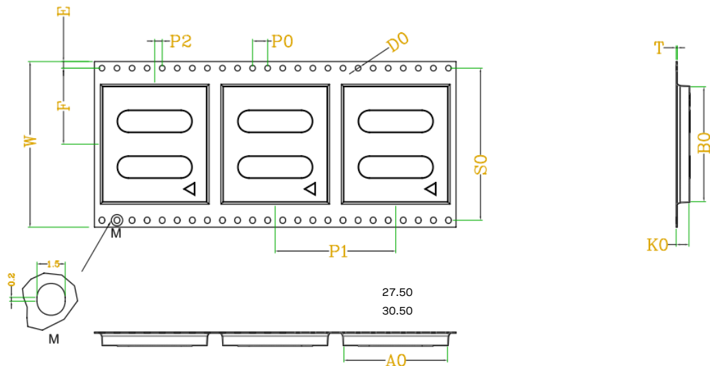
Figure 7: Orientation for LENA-R8 series modules on tape
