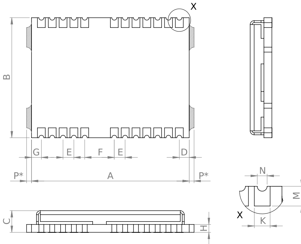
Figure 4 NEO-8Q mechanical drawing
