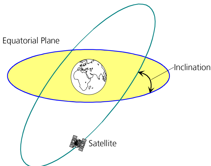
Figure 31: Satellite orbits
