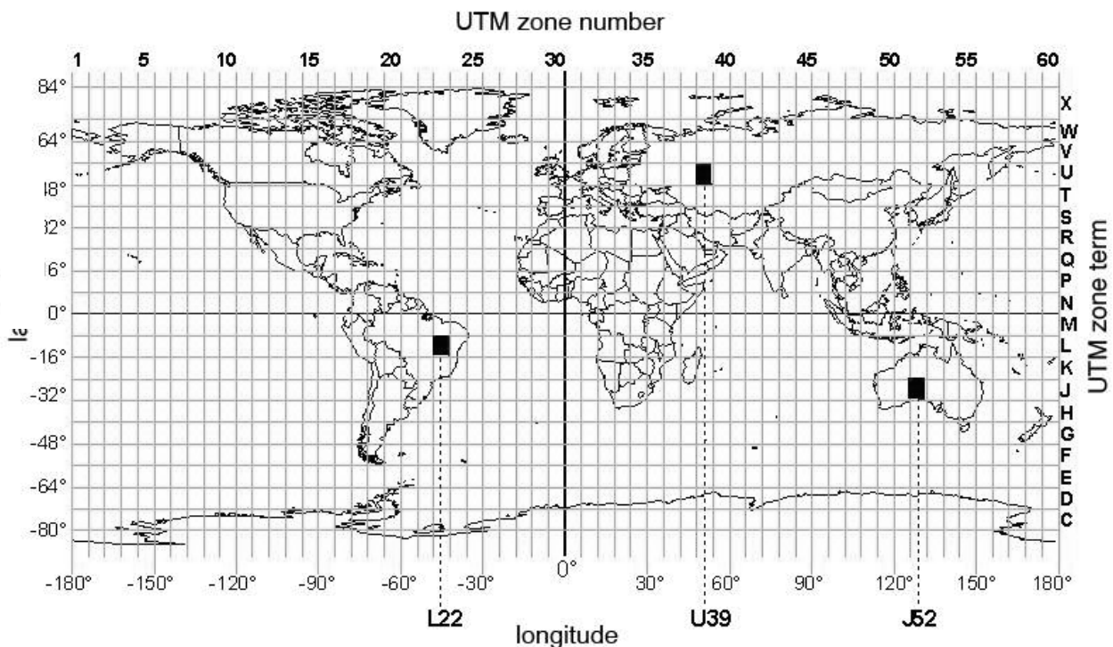
Figure 19: Designation of the zones using UTM, with examples
