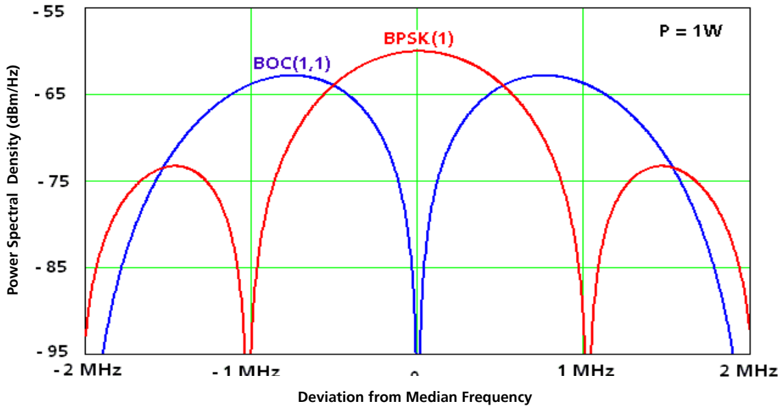
Figure 55: With BPSK(1) and BOC(1,1) the signal maxima are separated (signal strength normalized at 1 W per signal)
