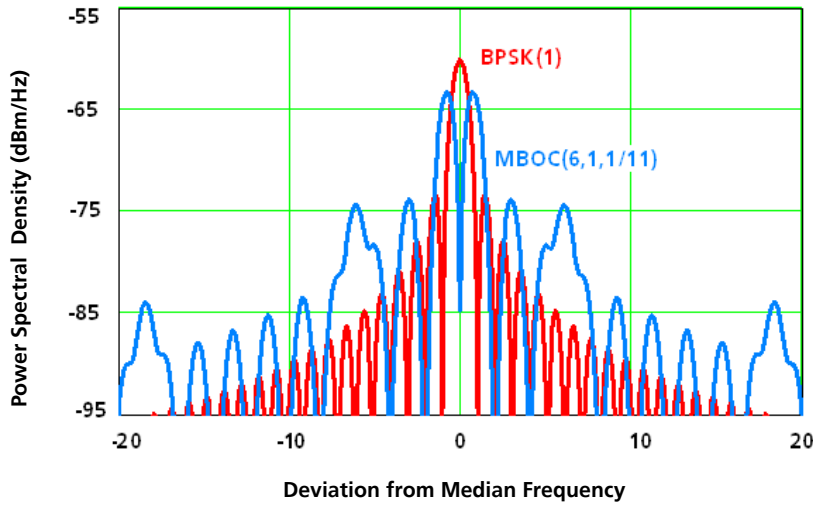
Figure 57: Power spectral density of MBOC(6,1,1/11) compared with BPSK(1) (P = 1W per signal)
