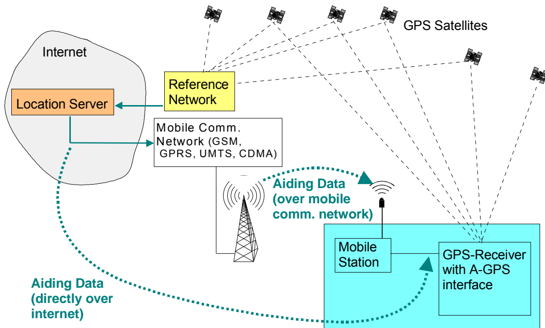
Figure 114: Assisted-GPS system
