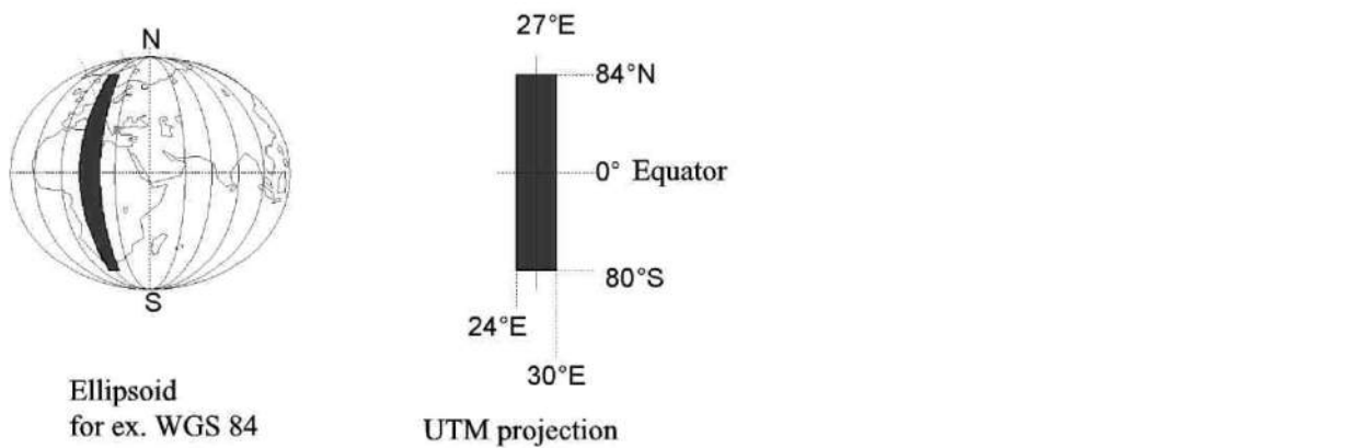
Figure 18: Principle of projecting one zone (of sixty)
