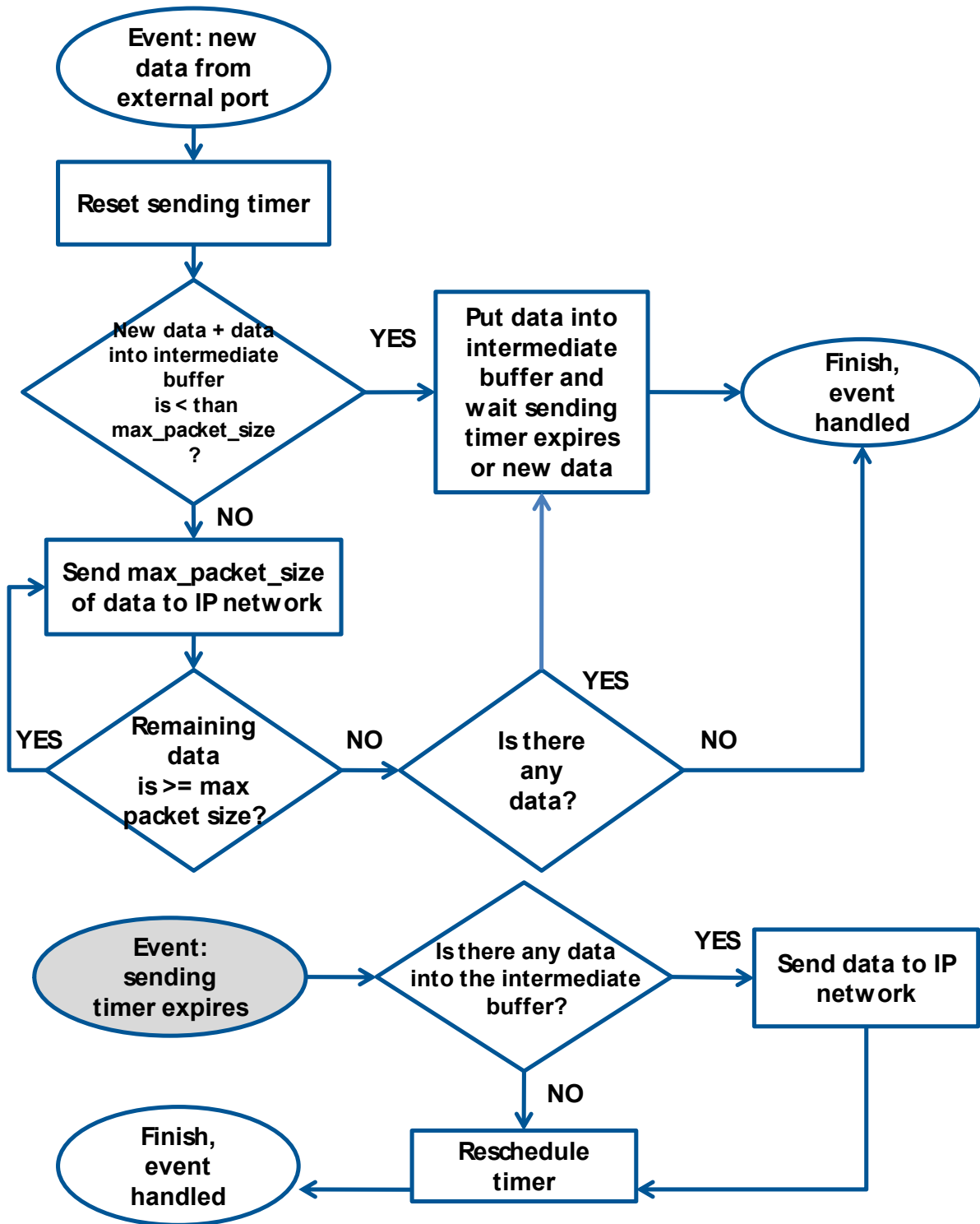
Figure 32: Workflow of data from the external port to the IP network
