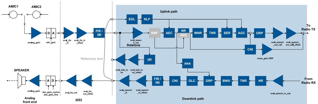
Figure 14: TOBY-L4 series audio analog path
