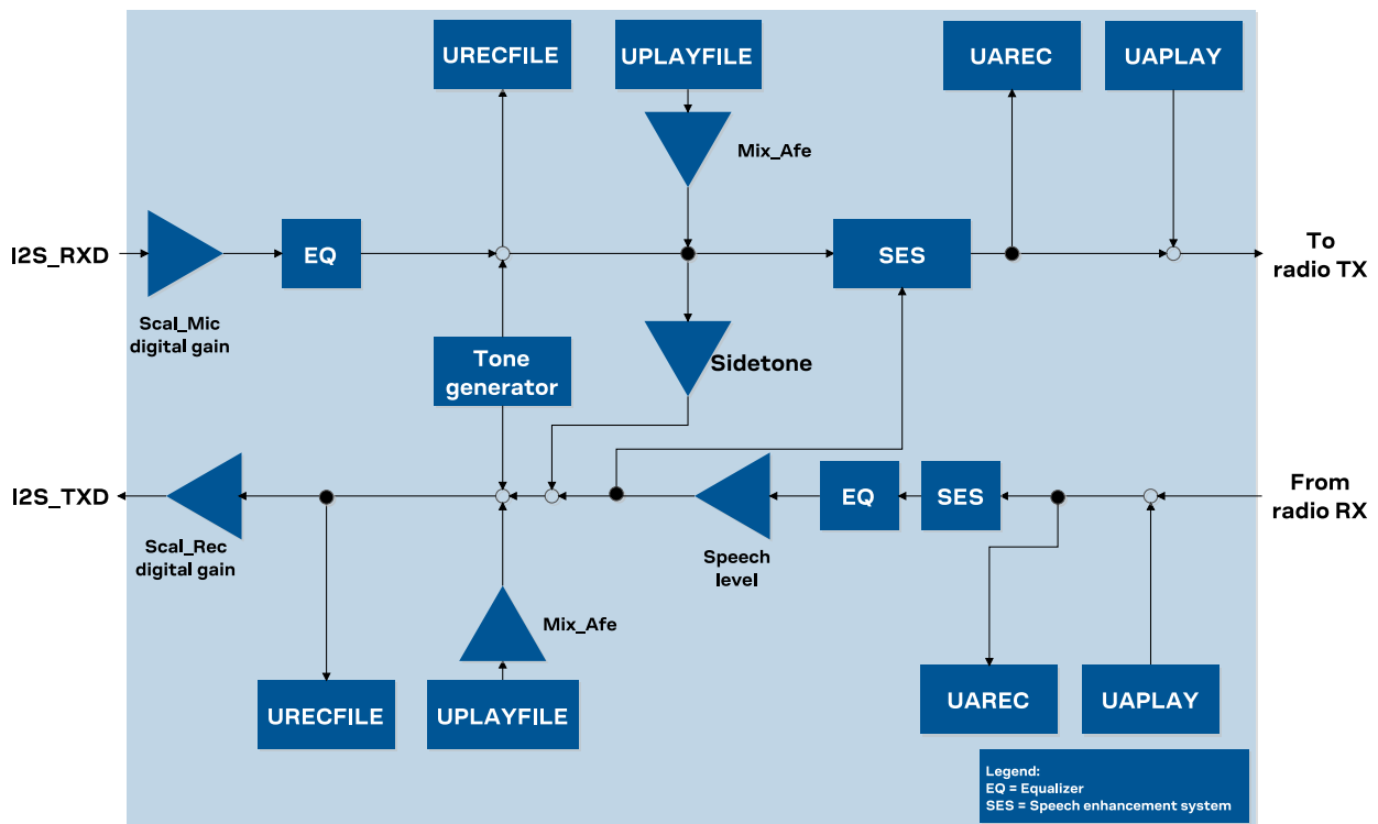
Figure 16: TOBY-R200 / TOBY-R202 / LARA-R202 / LARA-R203 / LARA-R211 audio paths
