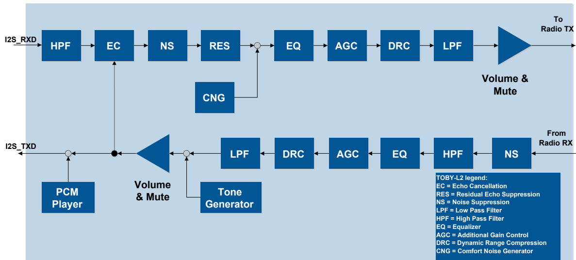
Figure 13: TOBY-L2 series audio paths
