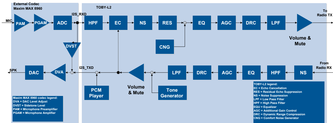
Figure 26: External codec controls
