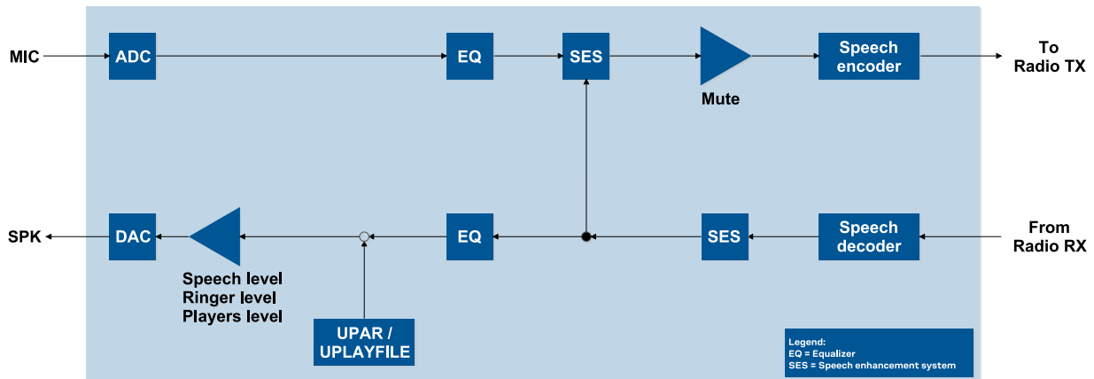
Figure 23: SARA-G4 series audio paths
