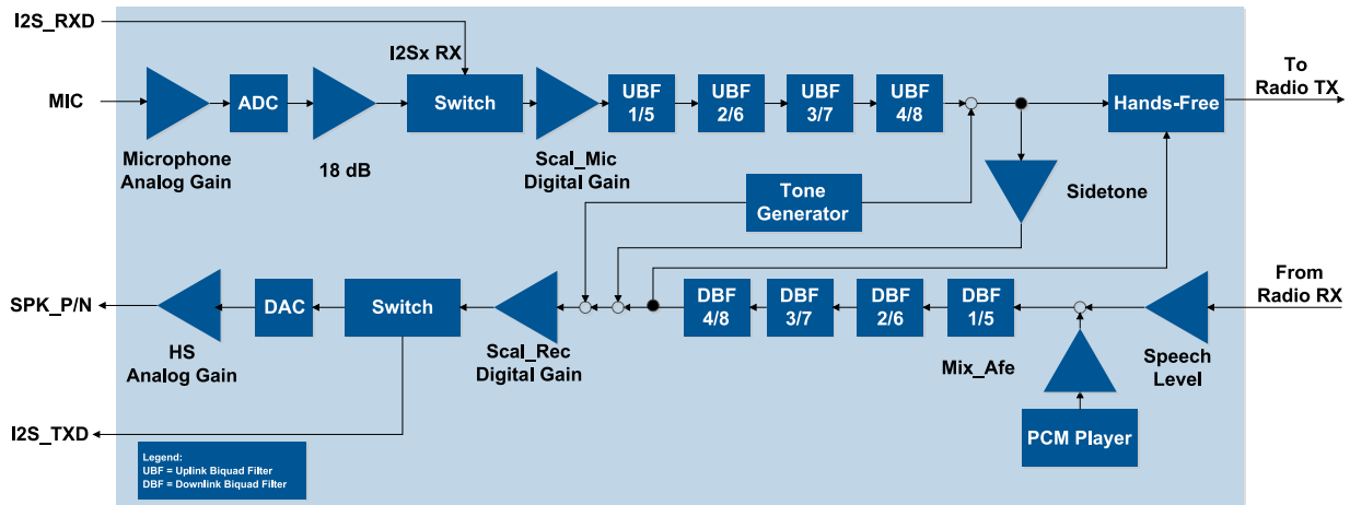
Figure 22: LISA-U1 series audio paths
