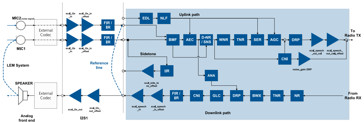
Figure 15: TOBY-L4 series audio digital path
