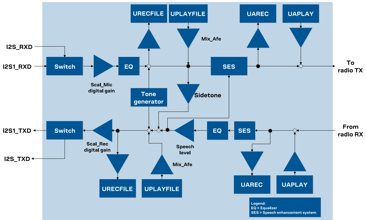
Figure 20: Audio paths of LISA-U2 "04" product versions
