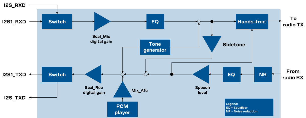
Figure 21: Audio paths of LISA-U2 "00", "01", "02", "03", "52", "62", "63", "68", "82", "83" product versions
