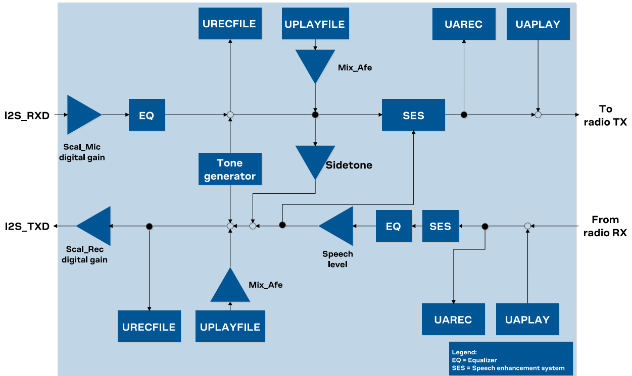
Figure 18: Audio paths of SARA-U2 "04" product versions
