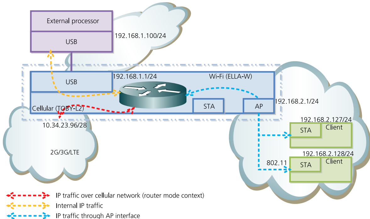
Figure 27: Router mode with Internet access via cellular network
