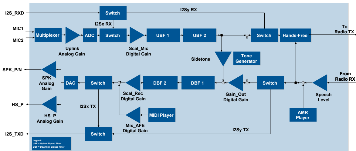
Figure 25: LEON-G1 series audio paths
