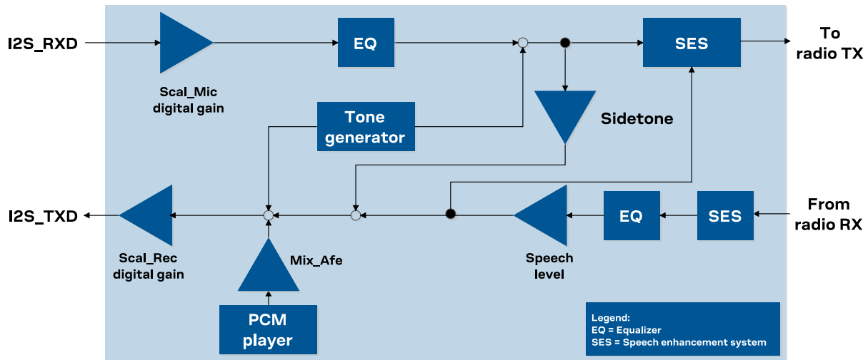
Figure 19: Audio paths of SARA-U2 "00", "03", "53", "63", "73" product versions
