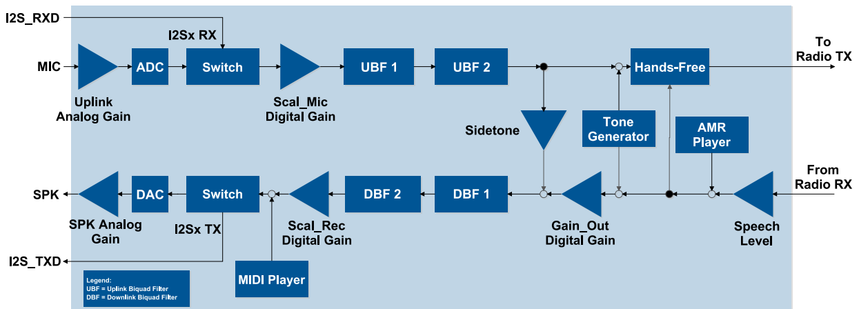
Figure 24: SARA-G3 series audio paths
