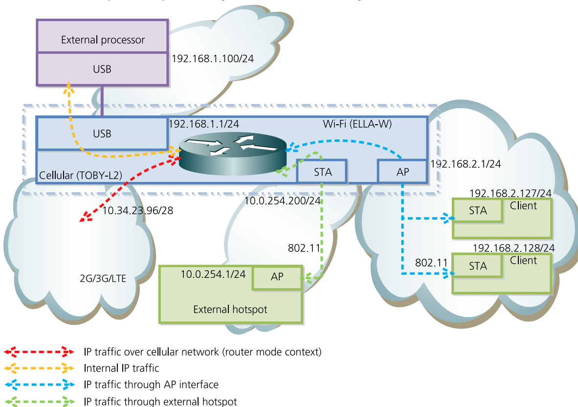
Figure 29: Router mode with Internet access via cellular network or via external hotspot
