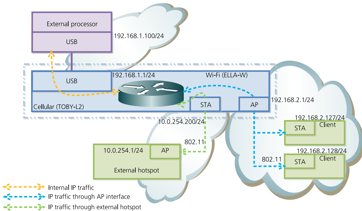
Figure 28: Router mode with Internet access via external hotspot
